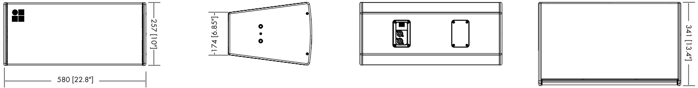
Yi10P cabinet dimensions in mm [inch]
