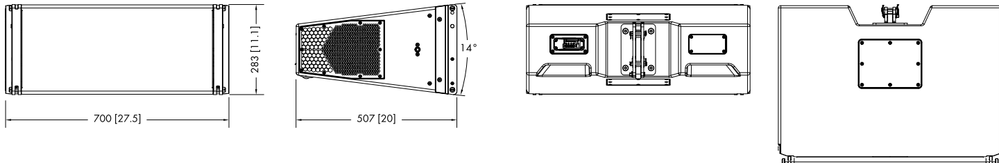
XSLi8 寸法 mm [inch]
