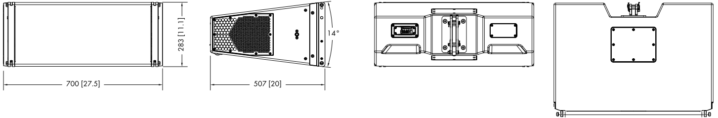
XSLi12 寸法 mm [inch]
