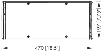
Ti10L cabinet dimensions in mm [inch]
