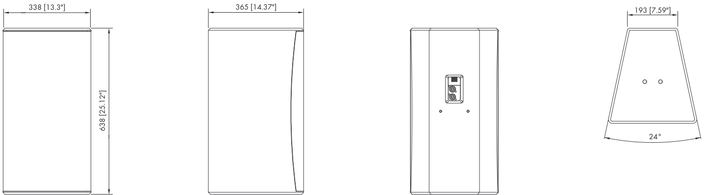
12S-D cabinet dimensions in mm [inch]
