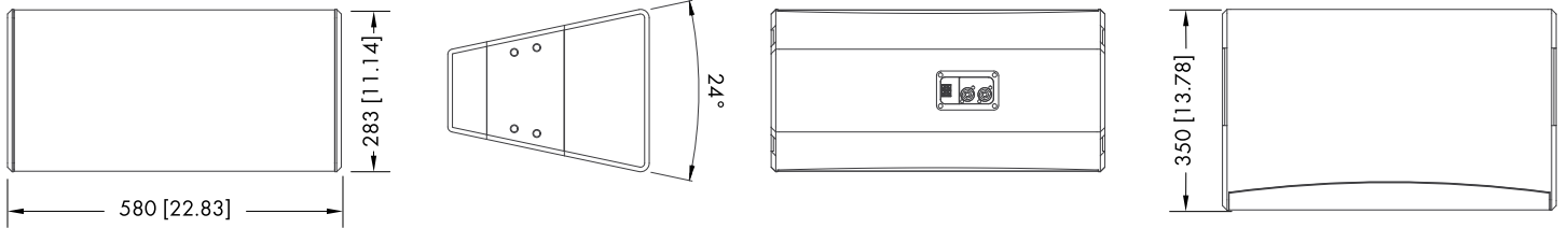
10A cabinet dimensions in mm [inch]
